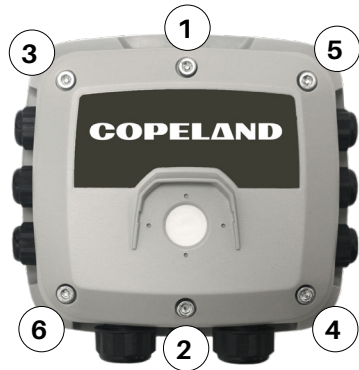
Tightening Pattern
