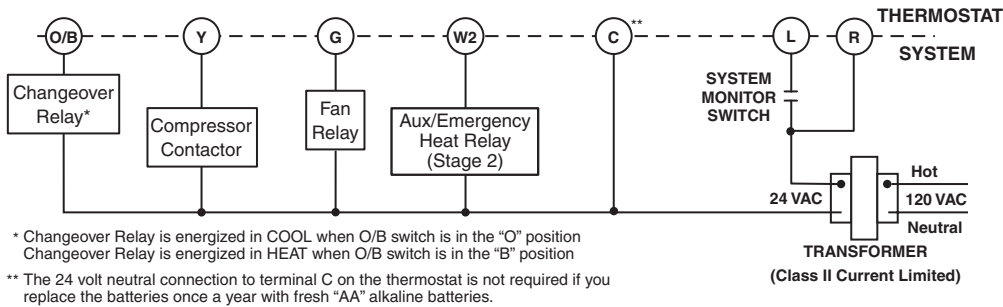
Figure 2. Typical wiring diagram for single transformer systems
