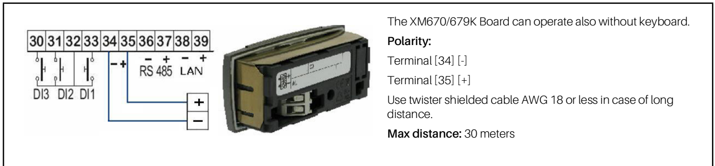
Figure 5-3 - Keyboard Display
