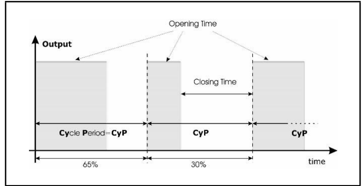
Figure 15-2 - Regulation Diagram
