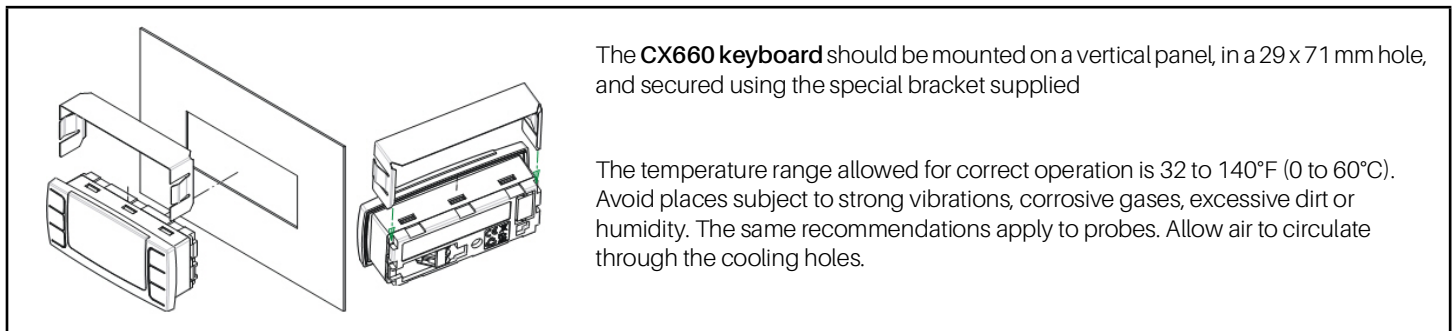
Figure 4-1 - CX660 Keyboard Installation and Mounting
