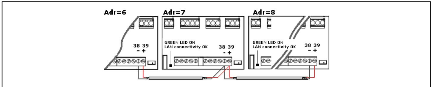
Figure 5-4 - LAN Connection
