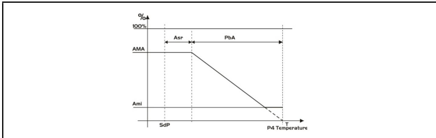
Figure 15-6 - Anti-Sweat Heaters
