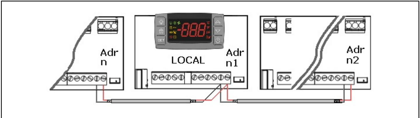
Figure 10-1 - LAN Connection
